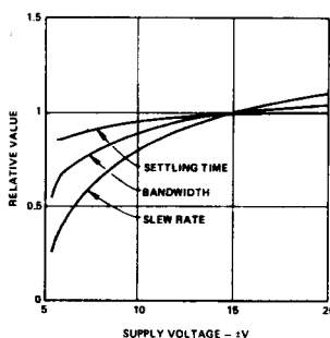
Figure 11. Dynamic Characteristics vs. Supply Voltage
